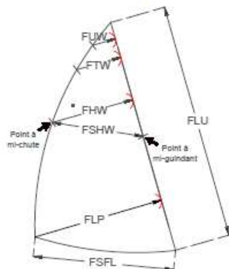
GENOIS VOLANT
